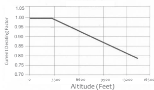
Altitude Derating Curve
