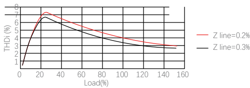
失真率和负荷率曲线 Distortion rate and load rate curve
